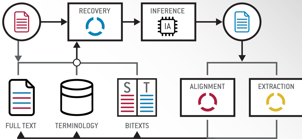
TAIGR flowchart
